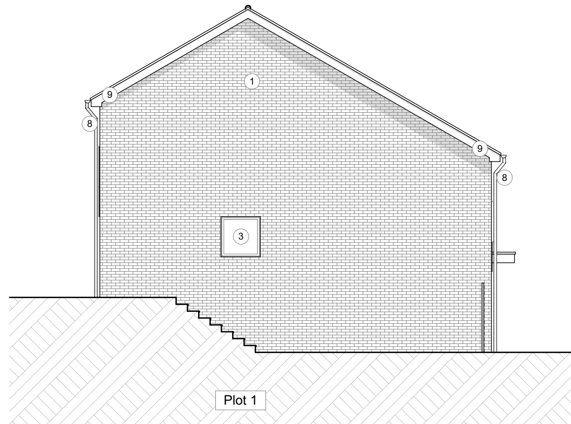
Side (Left) Elevation
