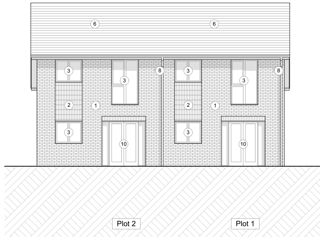
Rear Elevation
